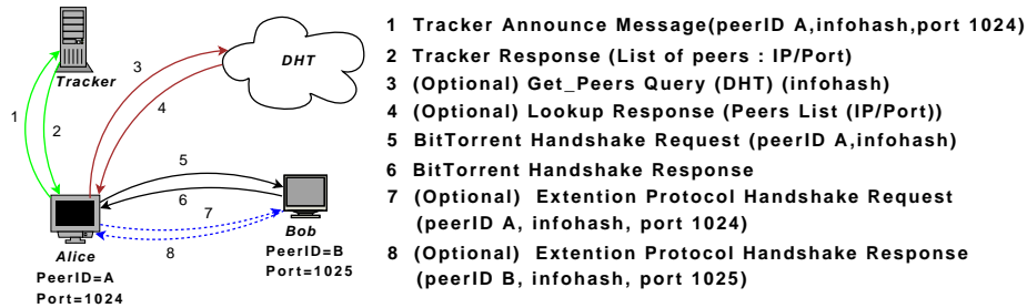
Fig. 1. BitTorrent Protocol Diagram
