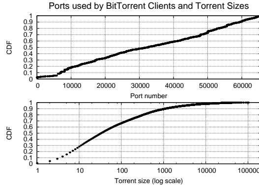
Fig. 2. Distribution of the listening ports used by the BitTorrent clients that we have de-anonymized on 6 monitored exit nodes during 23 days (top). Distribution of the torrent sizes in which peers using those exit nodes were participating in during the same period (bottom). Because the port numbers are uniformly distributed and most torrents are small, the port number is a good peer identifier.
