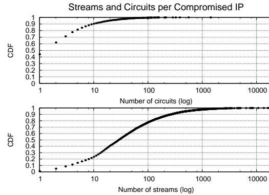
Fig. 3. Distribution of de-anonymized circuits (top) and streams (bottom) per de-anonymized IP. Once we de-anonymize an IP, we are able to de-anonymize multiple circuits and streams using the domino effect.
