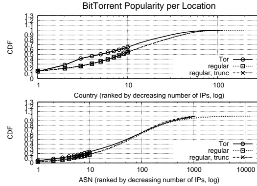
Fig. 6. Distribution of IPs per country (top) and AS (bottom) for the BitTorrent users on top of Tor (solid line) and the regular BitTorrent users (hashed line). For both subfigures, we also show the CDF of users per country (resp. AS) in regular BitTorrent with the number of countries (resp. ASes) truncated to be the same as in Tor (dash-dot line).
