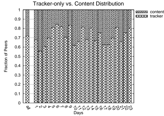
Fig. 4. For each day, this histogram shows the proportion of peers who use Tor for content distribution (content) or only to connect to the tracker (tracker). all is the average over all days. 72% of peers use Tor only to connect to the tracker.
