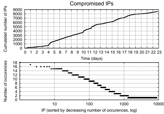
Fig. 5. Number of unique IPs that we de-anonymized in time (top) and number of occurrences of a de-anonymized IP with at least one day of interval (bottom). We compromised IPs uniformly in time. Whereas we de-anonymized most IPs once, a few IPs were de-anonymized many times.
