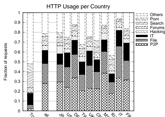
Fig. 7. Histogram of the HTTP usage per country. Tor represents the overall distribution of requests per category for all Tor users. all represents the overall distribution of requests per category for de-anonymized users. The country codes represent the same information but for each of the top10 countries in number of requests.
