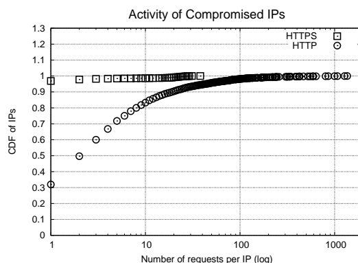
Fig. 8. CDF of compromised IP addresses establishing HTTP/HTTPS connections.
